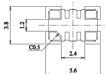
8 Land Pattern
